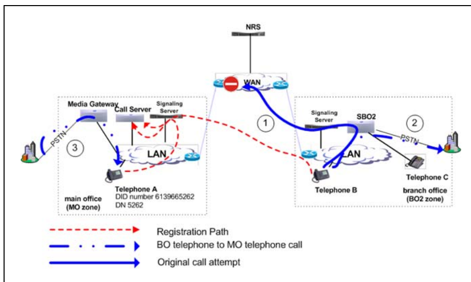
Figure 66 Call between a branch office telephone in Normal Mode and a main office telephone
